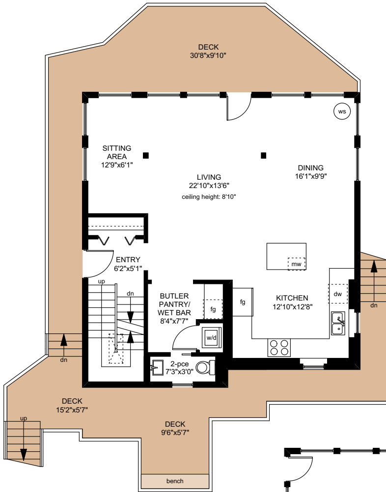
MAIN FLOOR 974 SQ.FT
