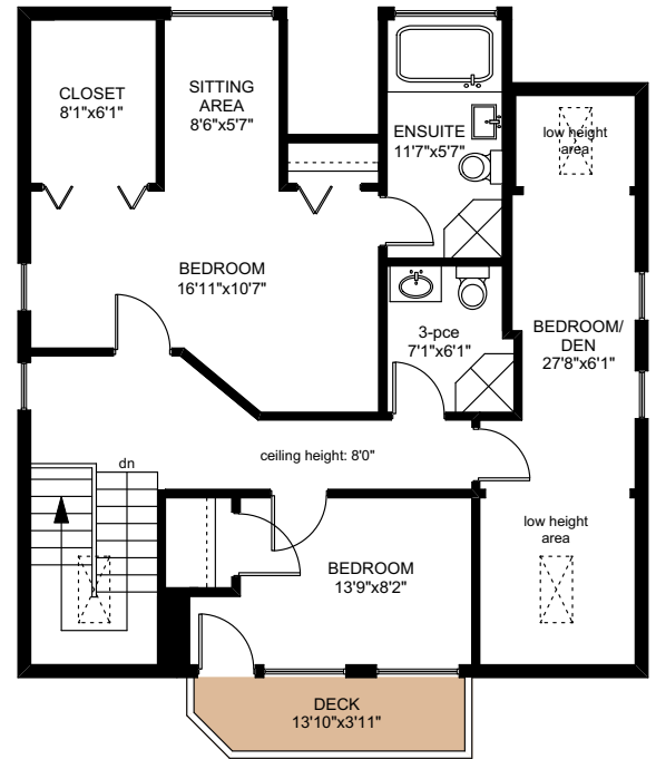
UPPER FLOOR 951 SQ.FT
